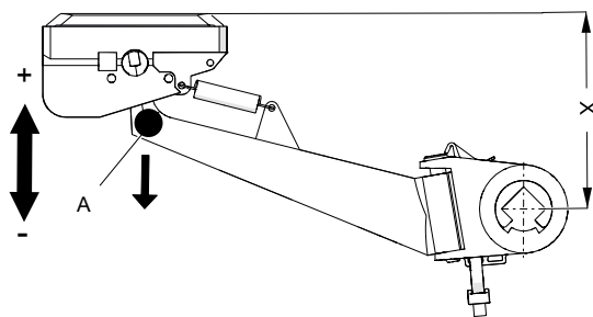
Illustration of the lateral tolerance
