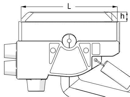
Illustration of conductor contact length and wear height 083106, 083107
